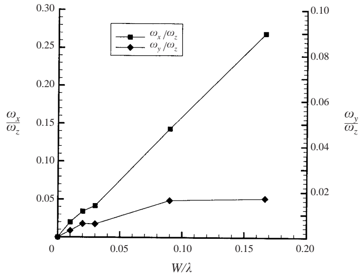
FIGURE 18. Variation of \omega_x/\omega_z and \omega_y/\omega_z with increasing wave steepness W/\lambda for \lambda/D = 5.6 .
